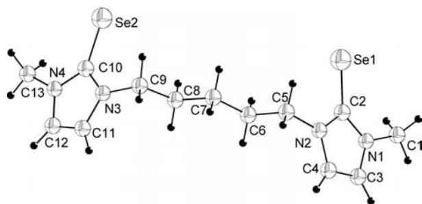
Figure 1. ORTEP representation at 50% probability and atom numbering scheme for Pbis in Pbis·H 2 O. Selected bond lengths [Å] and angles (°): Se1–C2 1.854(3), Se2–C10 1.848(3), N2–C2–N1 105.6(2), N2–C2–Se1 127.27(18), N1–C2–Se1 127.09(19), N3–C10–N4 105.6(2), N3–C10–Se2 127.23(18), N4–C10–Se2 127.16(18).
