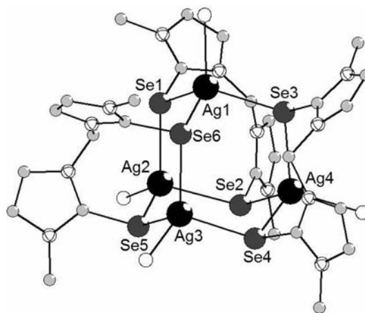
Figure 9. Molecular structure of the complex cation [Ag 4 (PPh 3 ) 4 -(Mbis) 3 ] 4+ in 18 , all hydrogen atoms, phenyl groups from PPh 3 and counter anions are omitted for clarity. Selected bond lengths [Å] and angles (°): Ag1–Se1 2.6603(7), Ag1–Se3 2.6693(7), Ag1–Se6 2.7251(7), Ag2–Se5 2.6818(7), Ag2–Se1 2.6885(7), Ag2–Se2 2.6937(7), Ag3–Se6 2.6440(7), Ag3–Se4 2.6819(7), Ag3–Se5 2.7151(7), Ag4–Se3 2.6377(7), Ag4–Se2 2.6747(7), Ag4–Se4 2.6815(7), Se1–Ag1–Se3 108.18(2), Se1–Ag1–Se6 111.637(19), Se3–Ag1–Se6 104.69(2), Se5–Ag2–Se1 104.29(2), Se5–Ag2–Se2 102.40(2), Se1–Ag2–Se2 106.40(2), Se6–Ag3–Se4 109.66(2), Se6–Ag3–Se5 108.58(2), Se4–Ag3–Se5 97.019(19), Se3–Ag4–Se2 108.23(2), Se3–Ag4–Se4 109.41(2), Se2–Ag4–Se4 101.75(2).
