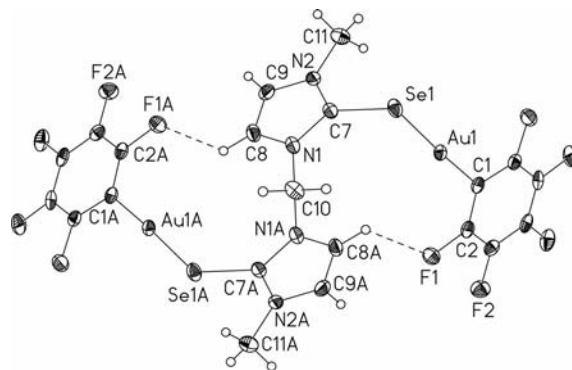
Figure 3. ORTEP representation at 50% probability and atom numbering scheme for 2 . Selected bond lengths [Å] and angles (°): Au1–C1 2.035(3), Au1–Se1 2.4263(5), Se1–C7 1.894(4), C1–Au1–Se1 177.49(10), C7–Se1–Au1 97.84(10), N1–C10–N1 109.6(4).
