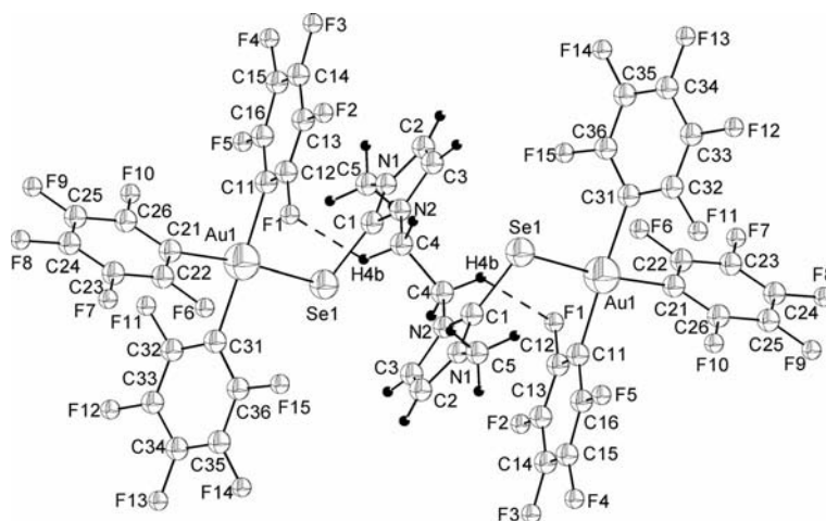
Figure 5. ORTEP representation at 50% probability and atom numbering scheme for 7 . Selected bond lengths [Å] and angles ( ^\circ ): Au1–C21 2.043(3), Au1–C11 2.052(3), Au1–C31 2.061(3), Au1–Se1 2.4607(6), Se1–C1 1.884(3), C21–Au1–Se1 173.43(9), C11–Au1–Se1 97.69(8), C31–Au1–Se1 85.09(8), C21–Au1–C11 88.83(12), C21–Au1–C31 88.40(12), C1–Se1–Au1 103.58(9).
