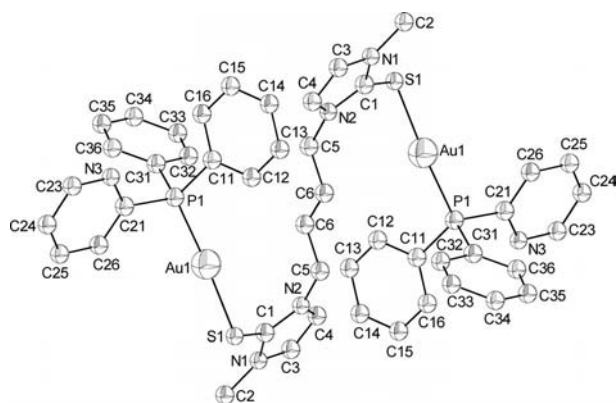
Figure 7. ORTEP representation at 50% probability and atom numbering scheme for the complex cation [Au 2 (PPh 2 py) 2 (Bbit)] 2+ in 13 . All hydrogen atoms, counter anions and solvents (CH 2 Cl 2 ) are omitted for clarity. Selected bond lengths [Å] and angles (°): Au1–S1 2.313(2), S1–C1 1.726(9), Au1–P1 2.264(2), P1–Au1–S1 173.77(7), C1–S1–Au1 106.5(3), N1–C1–S1 124.4(8), N2–C1–S1 128.1(8).
